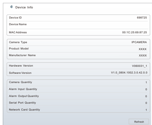
Figure3-6 Device Info
