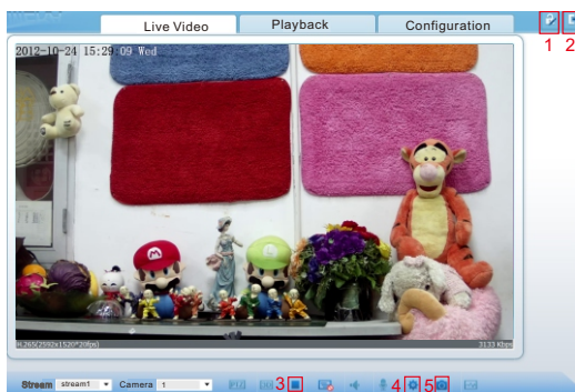
Figure 3-5 Live Video
