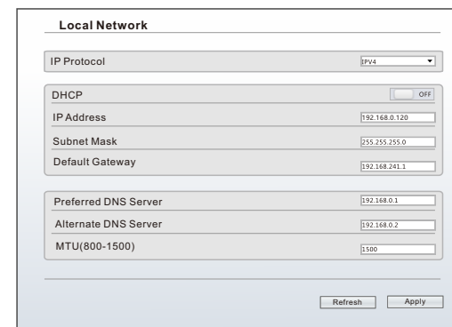
Figure 3-2 Local Network
