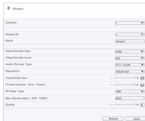
Figure3-7 Stream
