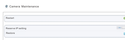
Figure3-8 Camera Maintenance
